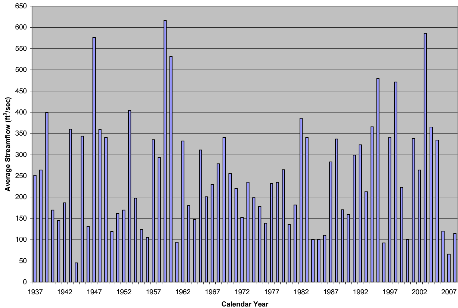
FIGURE 6 – Average Historical Streamflow at USGS Sarasota Gauge 1937-2008
